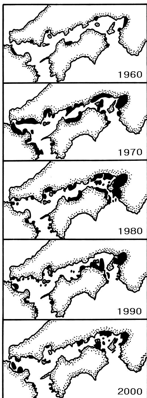
Fig. 5. Decadal changes in the distribution of red-tide areas in the Seto Inland Sea.
