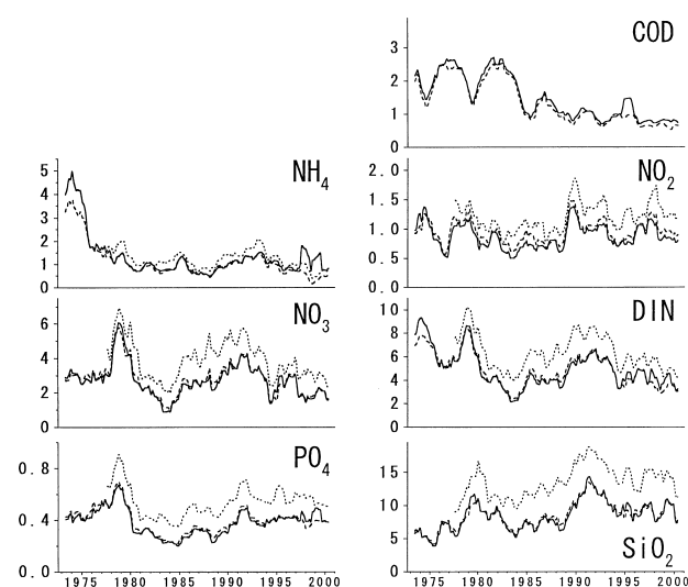
Fig. 3. Long-term changes in COD ( \text{mgL}^{-1} ) and nutrients ( \mu\text{M} ) in the north-eastern part of Harima-Nada, the Seto Inland Sea (solid lines: surface, dashed lines: 10 m, dotted lines: bottom) from April 1973 to March 2000. Data were treated by 12-month moving average process.
