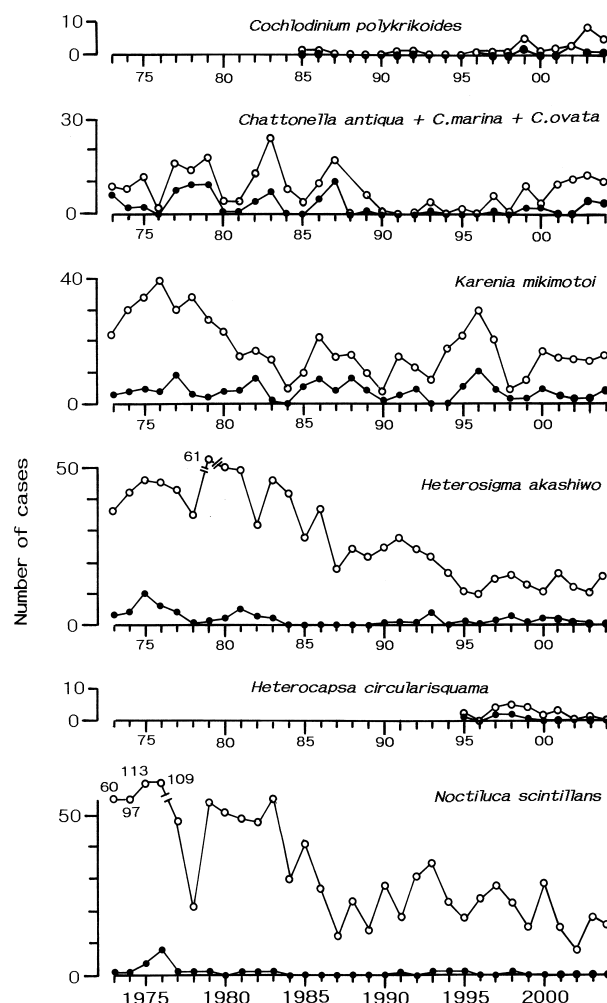
Fig. 6. Number of red tides (open circle) and those with fishery damage (closed circle) caused by Cochlodinium polykrikoides , Chattonella spp., Karenia mikimotoi , Heterosigma akashiwo , Heterocapsa circularisquama , and Noctiluca scintillans in the Seto Inland Sea from 1973 to 2004.
