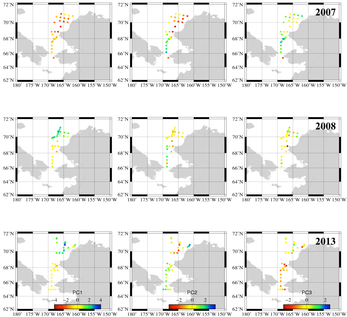
Figure 3. Distribution of main principal component score (PC1–3) in 2007, 2008 and 2013. Coloured circles indicate magnitude of PC.
