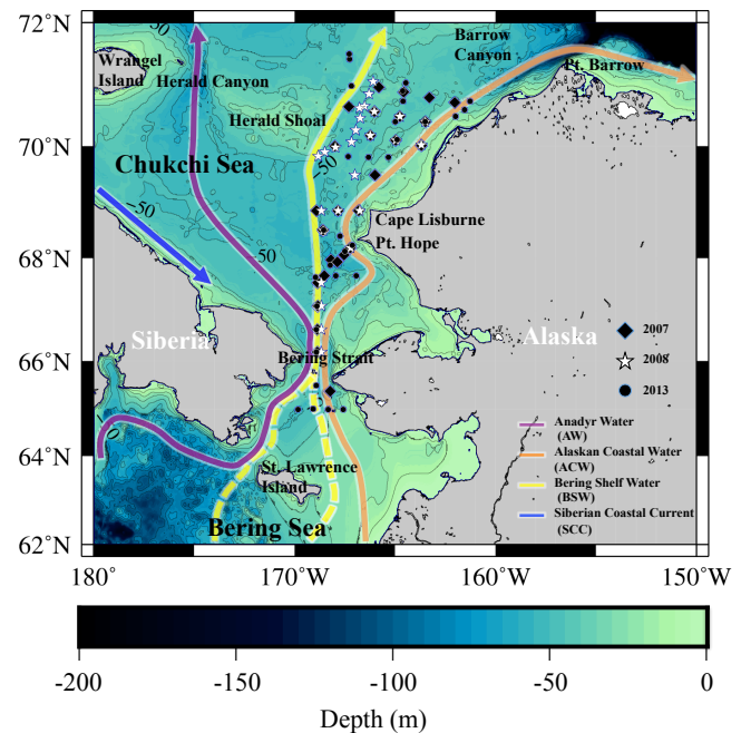
Figure 1. Study area and sampling stations in the northern Bering and Chukchi seas during the summers of 2007, 2008 and 2013. The symbols denote the sampling stations where NORPAC net and CTD water samplings were conducted. Modified from figure presented in Spall et al. (2014) and Grebmeier et al. (2015).
