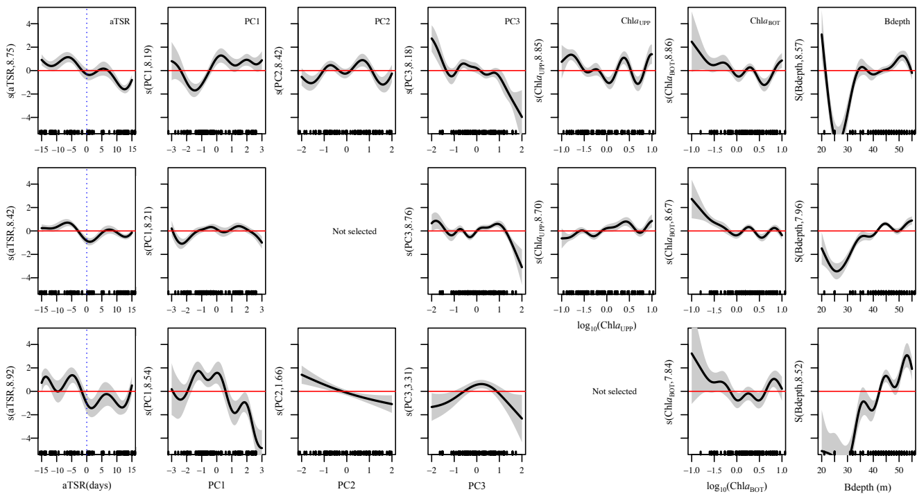
Figure 5. GAM plot of the best model in each copepod groups: large Arctic ( CopL_{arc} ), small Arctic ( CopS_{arc} ) and Pacific ( CopP_{ac} ) copepods. The horizontal axes show the explanatory variable: the anomaly of the timing of sea ice retreat (aTSR), principal component score (PC1–3) averaged log-transformed chlorophyll a concentration within the layer above and below pycnocline, ( Chl a_{UPP} and Chl a_{BOT} ) and bottom depth (Bdepth). Shade area represents 95 % confidence intervals. The vertical axes indicate the estimate smoother for the abundance of copepods. The estimated smoother converts the explanatory variable to fit the models, so it shows positive effects for response variables and the magnitude of its effects when estimated smoother is positive and vice versa. Short vertical lines located on the x axes of each plot indicate the values at which observations were made.
