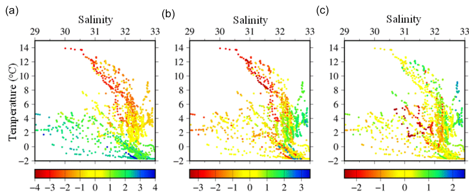
Figure 2. T - S diagrams of principal component scores (a) PC1, (b) PC2 and (c) PC3. Coloured circles indicate the magnitude of each PC.
