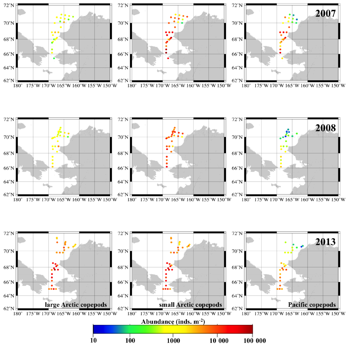
Figure 4. Distribution of copepods abundance in 2007, 2008 and 2013. large Arctic (Cop Larc ), small Arctic (Cop Sarc ) and Pacific (Cop Pac ) copepods.
