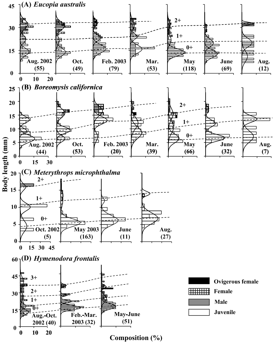
Fig. 4. Temporal changes at Site H from August 2002 to August 2003 in body length composition of A, Eucopia australis Dana, 1852; B, Boreomysis californica Ortmann, 1894; C, Meterythropters microphthalmum W. Tattersall, 1951; D, Hymenodora frontalis Rathbun, 1902. The number of individuals measured for each histogram is shown in parentheses. For D, data from several months were combined due to low abundance of this species. Dashed lines indicate estimated growth of each cohort.
