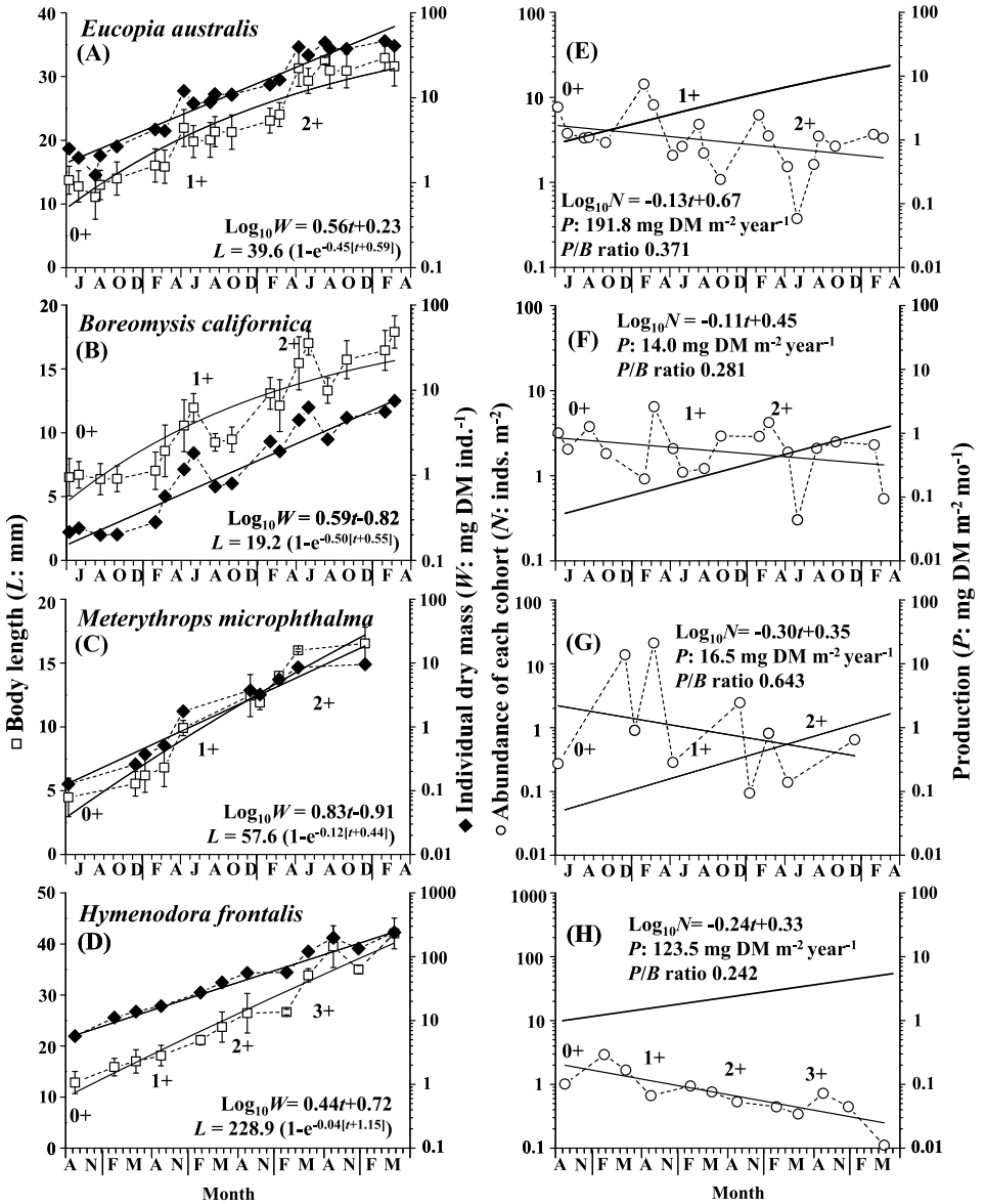
Fig. 5. Estimated growth curve for body length (open symbols) and dry mass (solid symbols) at Site H of A, Eucopia australis Dana, 1852; B, Boreomysis californica Ortmann, 1894; C, Meterythrops microphthalma W. Tattersall, 1951; D, Hymenodora frontalis Rathbun, 1902. Abundance of each cohort (open symbols) from body length histogram (cf. fig. 4) and estimated production (solid lines) of: E, E. australis ; F, B. californica ; G, M. microphthalma ; H, H. frontalis . Symbols and bars in A-D indicate means and standard deviations for each cohort. Annual production and production/biomass ( P/B ) ratios are also shown for E-H. t , time (year).
