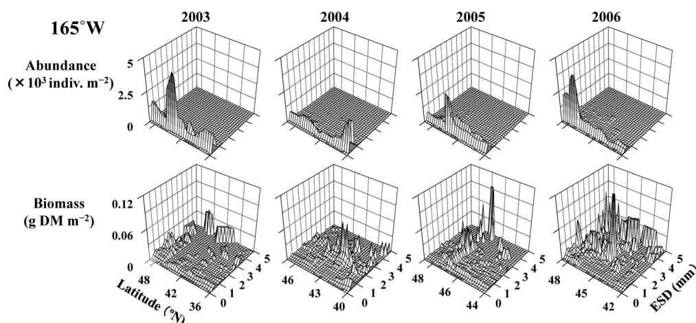
Fig. 6. Latitudinal changes in abundance and biomass with each size class along 165°W in the eastern North Pacific during summers of 2003–2006.
