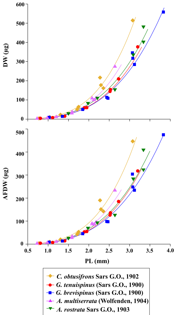
Fig. 1. Relationships between dry weight (DW) and prosome length (PL) (upper) and ash-free dry weight (AFDW) and PL (lower) for the five dominant aetideid copepods in the western Arctic Ocean: Chiridius obtusifrons Sars G.O., 1902, Gaetanus tenuispinus (Sars G.O., 1900), Gaetanus brevispinus (Sars G.O., 1900), Aetideopsis multiserrata (Wolfenden, 1904), and Aetideopsis rostrata Sars G.O., 1903. For details of the regressions, see tables II, IV, VI, VIII and X.
