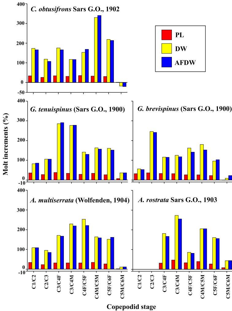
Fig. 3. Molt increments (MI) in prosome length (PL) and body weights (DW: dry weight, AFDW: ash-free dry weight) of the five dominant aetideid copepods in the western Arctic Ocean: Chiridius obtusifrons Sars G.O., 1902, Gaetanus tenuispinus (Sars G.O., 1900), Gaetanus brevispinus (Sars G.O., 1900), Aetideopsis multiserrata (Wolfenden, 1904), and Aetideopsis rostrata Sars G.O., 1903. F, female; M, male.
