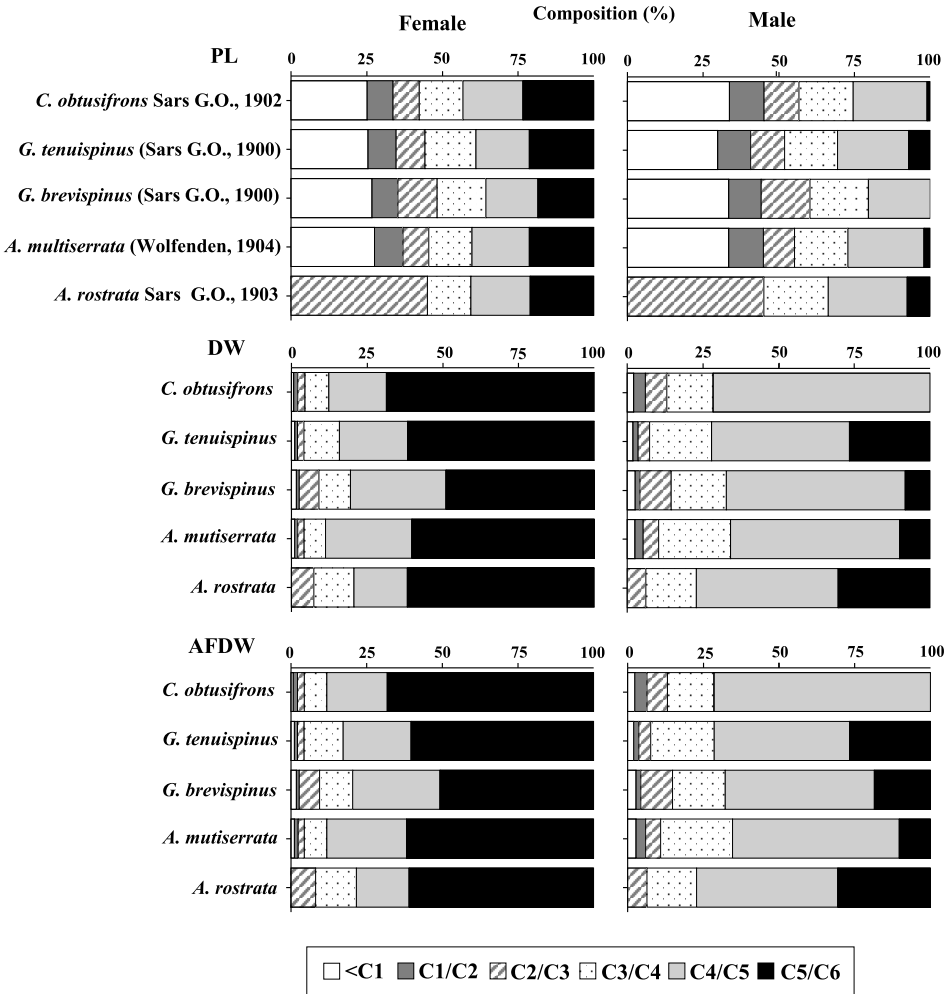
Fig. 4. The proportion of growth (PG) in prosome length (PL) and weights (dry weight (DW) and ash-free dry weight (AFDW)) at each stage, which is calculated by the C6 values as 100% for the five dominant arctideid copepods in the western Arctic Ocean: Chiridius obtusifrons Sars G.O., 1902, Gaetanus tenuispinus (Sars G.O., 1900), Gaetanus brevispinus (Sars G.O., 1900), Aetideopsis mutiserrata (Wolfenden, 1904), and Aetideopsis rostrata Sars G.O., 1903. Note that C1 and C2 were not available for Aetideopsis rostrata ; their C2/C3 stage is treated as <math><C_3</math>.
