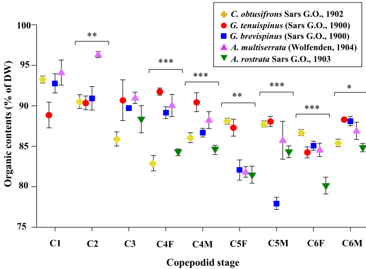
Fig. 2. Organic contents (% of DW) of the five dominant aetideid copepods in the western Arctic Ocean: Chiridius obtusifrons Sars G.O., 1902, Gaetanus tenuispinus (Sars G.O., 1900), Gaetanus brevispinus (Sars G.O., 1900), Aetideopsis multiserrata (Wolfenden, 1904), and Aetideopsis rostrata Sars G.O., 1903, at each copepodid stage. Symbols and bars represent means and standard errors, respectively. F, female; M, male. Inter-species differences were tested by one-way ANOVA for each stage. * p < 0.05 , ** p < 0.01 , *** p < 0.001 .
